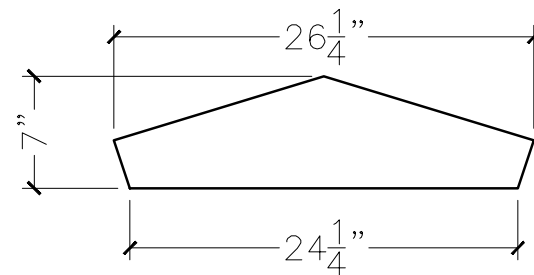
SECTION VIEW
