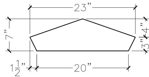
SECTION VIEW
