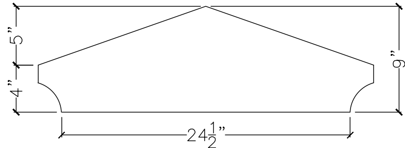
SECTION VIEW
