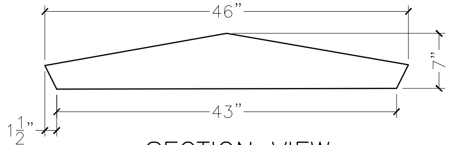
SECTION VIEW
