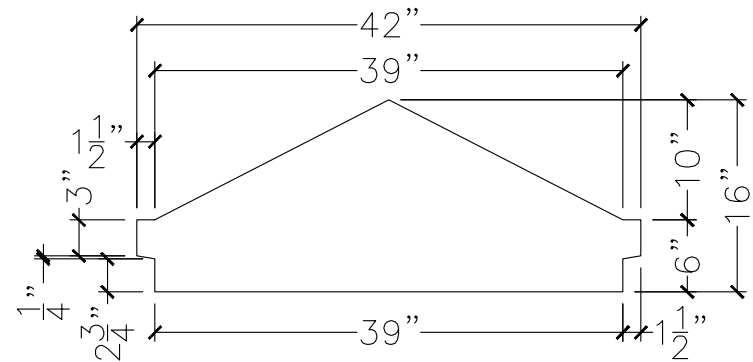
SECTION VIEW
