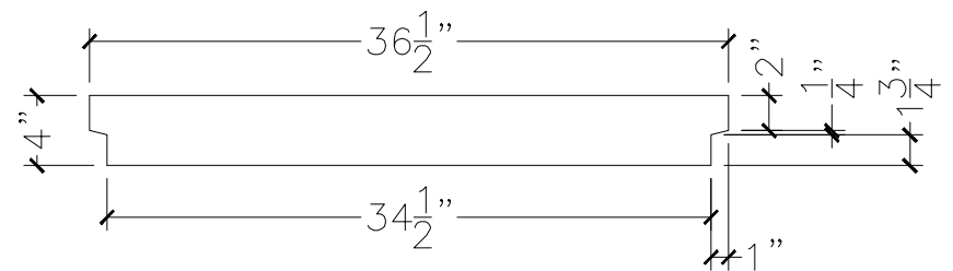
SECTION VIEW
