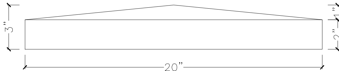
FRONT VIEW
