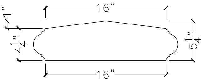
SECTION VIEW
