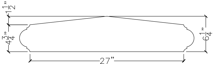
SECTION VIEW
