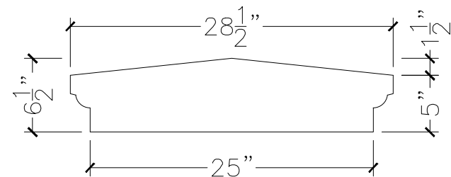
SECTION VIEW
