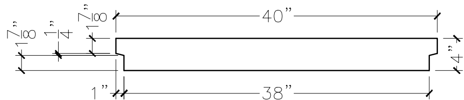
SECTION VIEW
