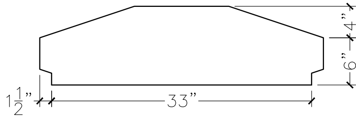
SECTION VIEW
