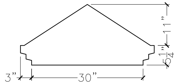
SECTION VIEW
