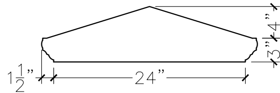
SECTION VIEW
