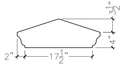
SECTION VIEW
