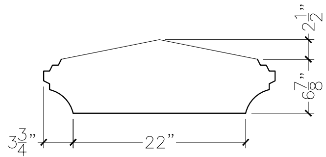
SECTION VIEW
