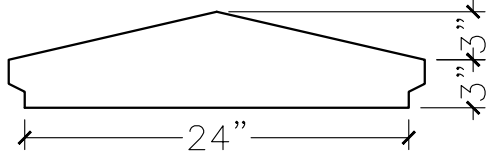
SECTION VIEW
