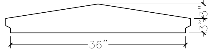
SECTION VIEW
