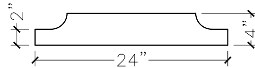
SECTION VIEW
