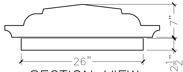
SECTION VIEW
