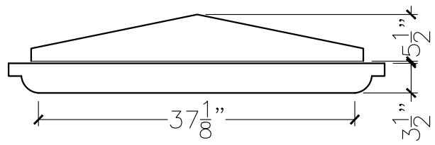
SECTION VIEW
