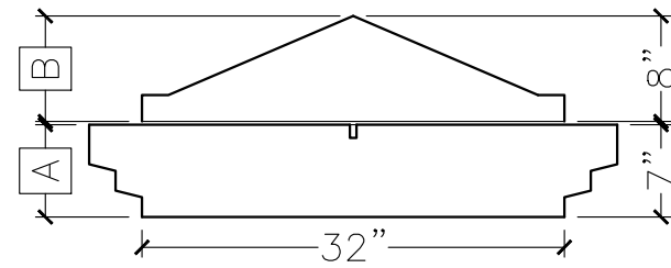
SECTION VIEW
