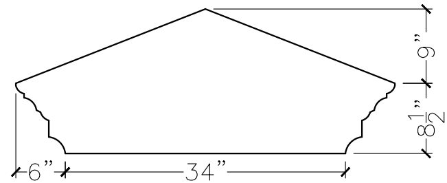
SECTION VIEW
