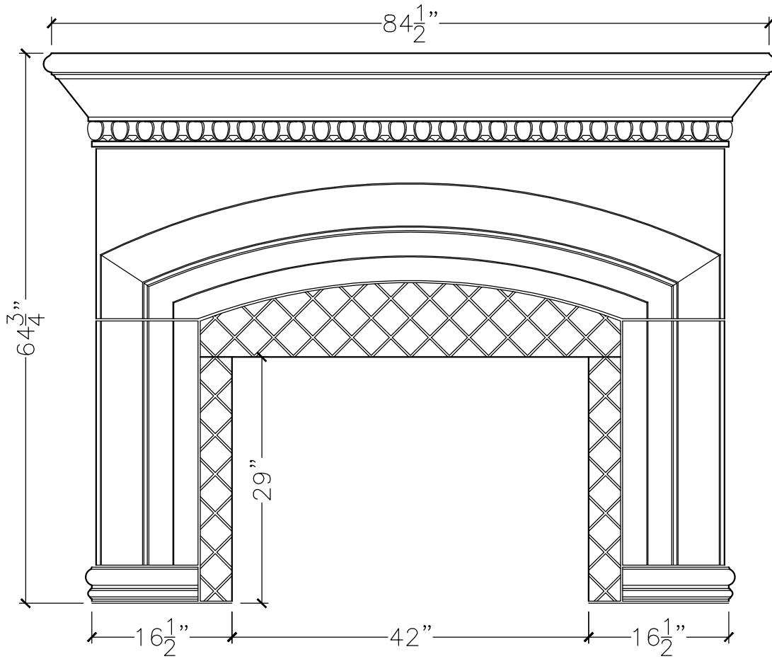
FRONT VIEW
