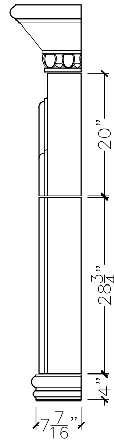
SIDE
