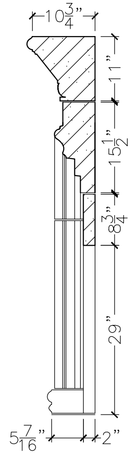
SECTION
