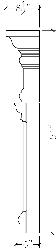
SIDE VIEW
