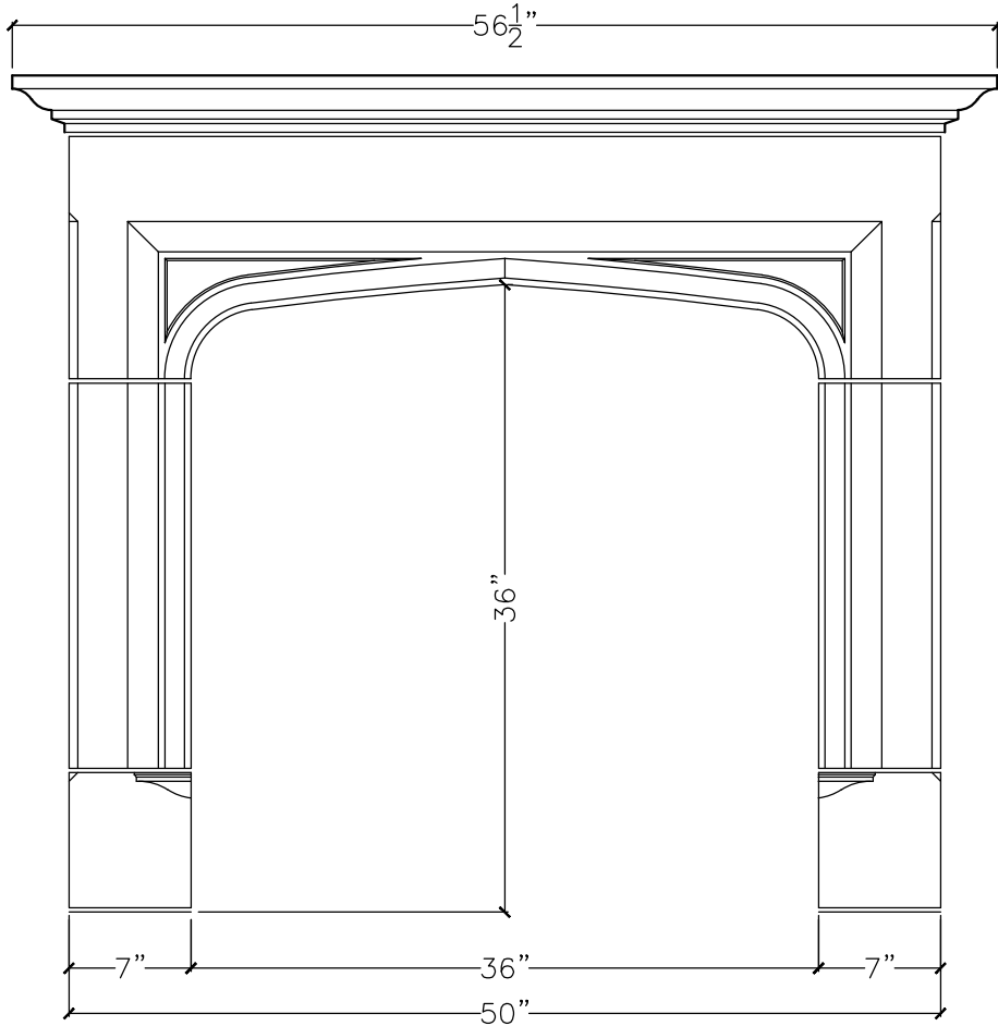
FRONT VIEW
