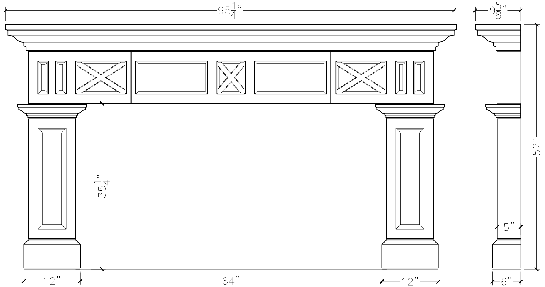
FRONT VIEW
