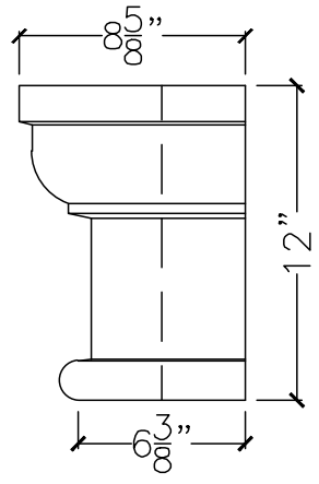
END VIEW
