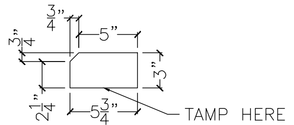
SECTION VIEW
