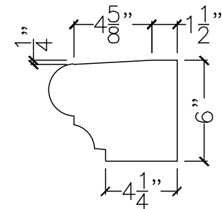
SECTION VIEW
