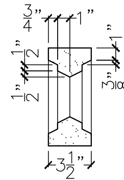
SECTION VIEW
