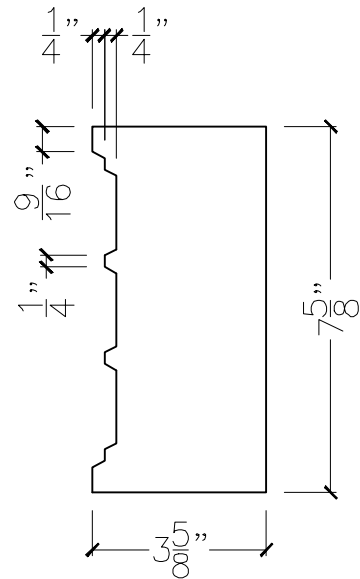
SECTION VIEW
