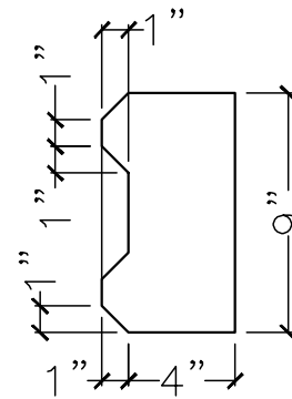
SECTION VIEW
