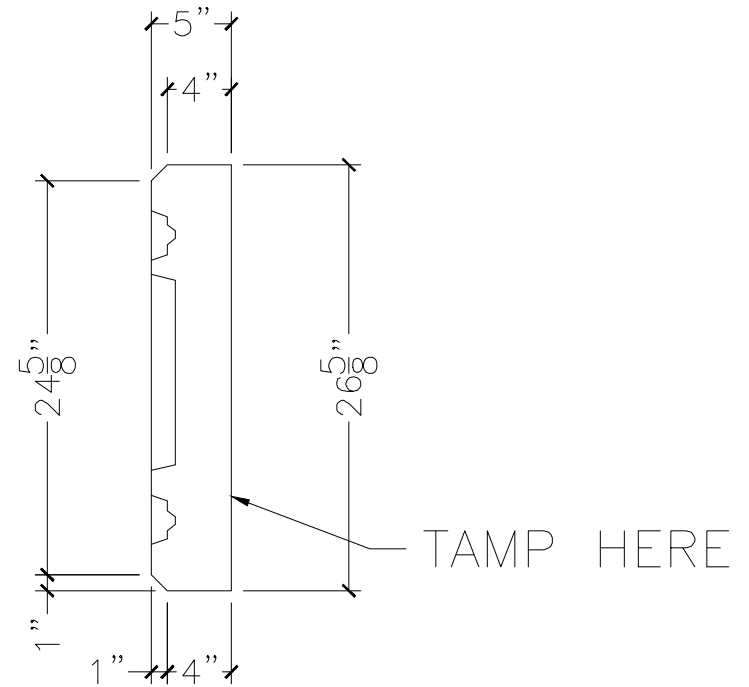
SECTION VIEW
