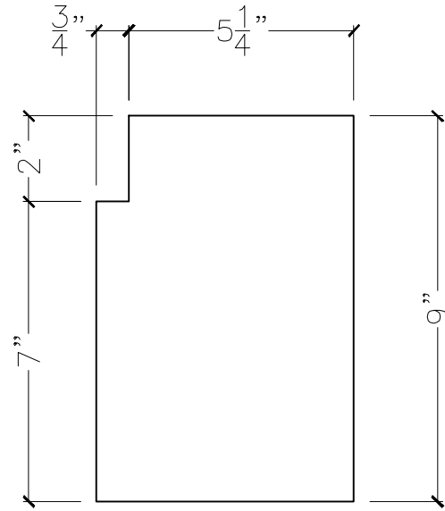
SECTION VIEW
