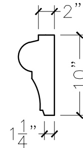
SECTION VIEW
