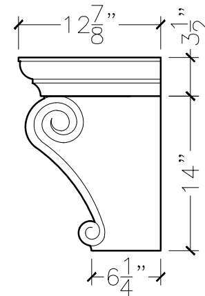
SECTION VIEW
