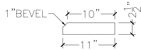
SECTION VIEW
