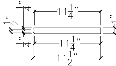
SECTION VIEW
