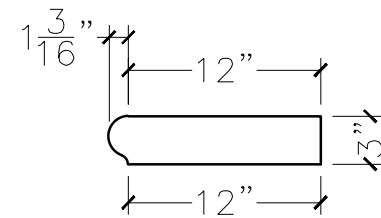
SECTION VIEW
