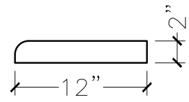
SECTION VIEW
