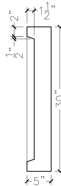
SECTION VIEW
