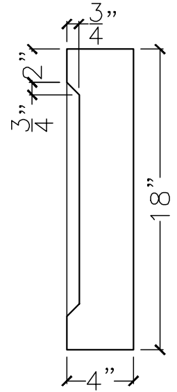
SECTION VIEW
