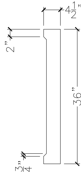
SECTION VIEW
