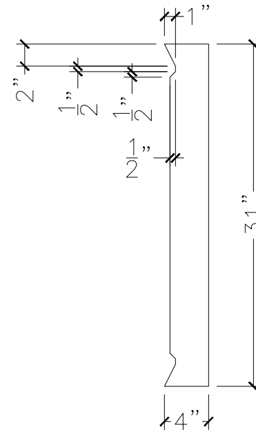
SECTION VIEW
