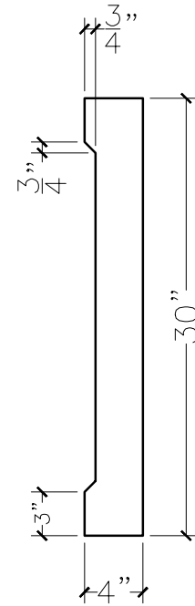
SECTION VIEW
