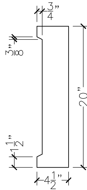
SECTION VIEW
