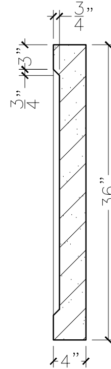
SECTION VIEW
