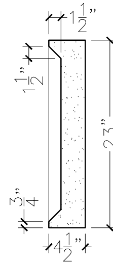
SECTION VIEW
