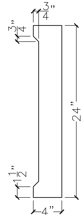
SECTION VIEW
